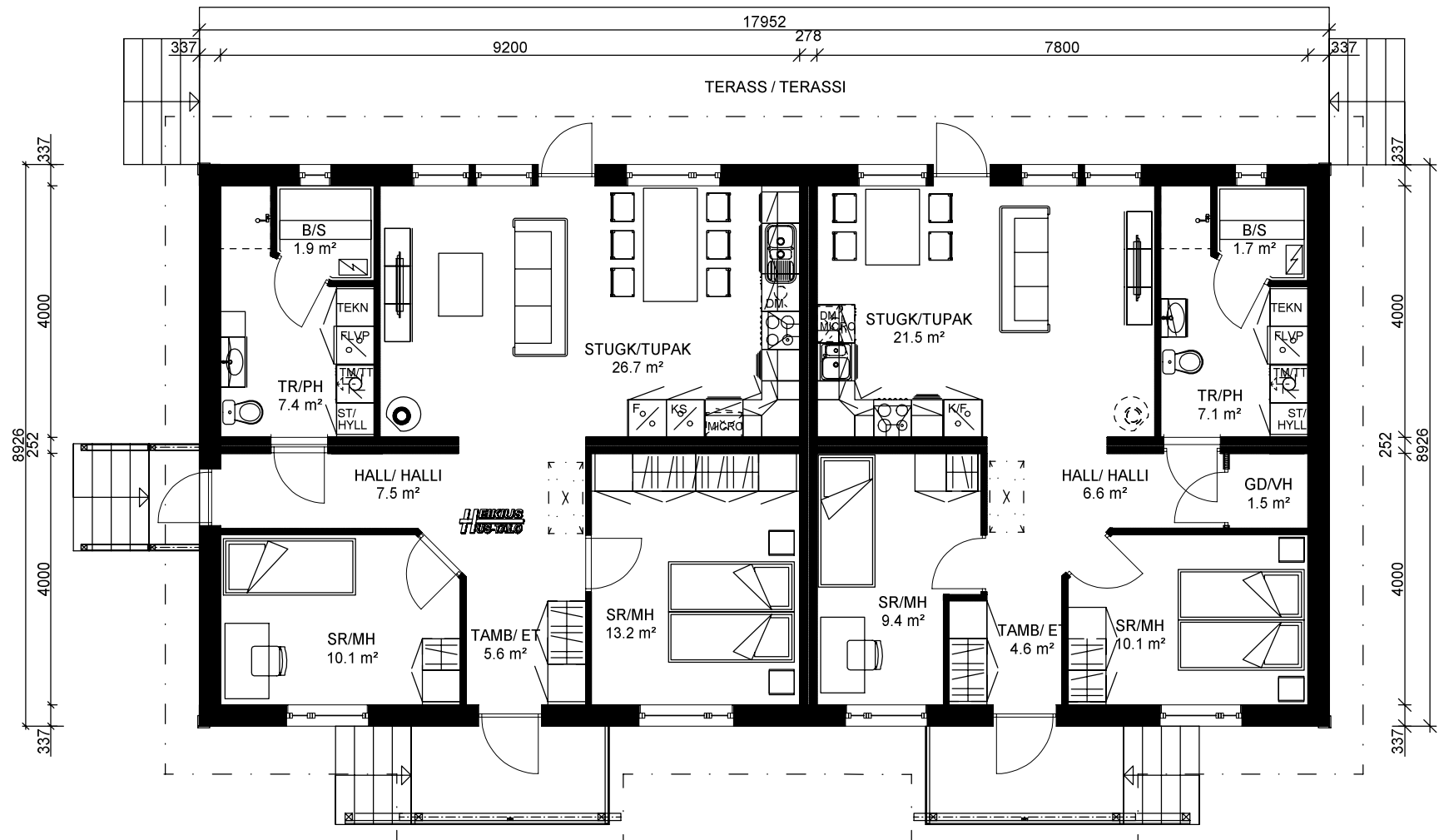
B3; 2 R + STUGA, 74,0m 2
